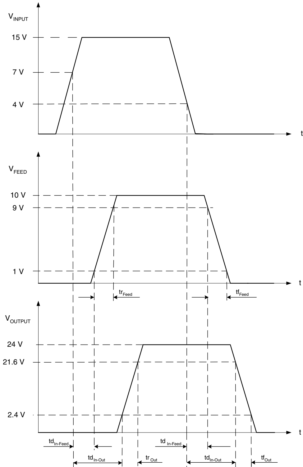
Figure 3. Timing Diagram (1)
